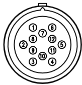
FACE VIEW SOCKET CONNECTOR
