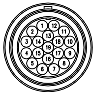
FACE VIEW SOCKET CONNECTOR
