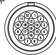
FACE VIEW PIN CONNECTOR
