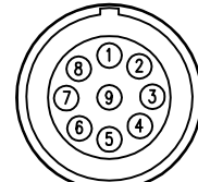
FACE VIEW PIN CONNECTOR
