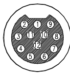
FACE VIEW SOCKET CONNECTOR
